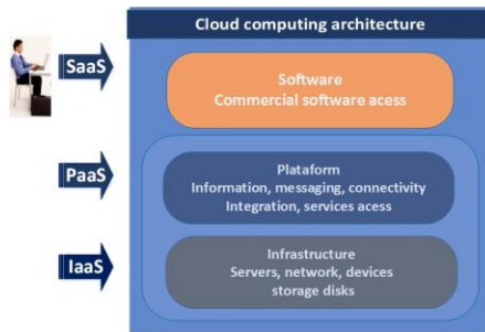
Figure 1: Cloud computing architecture [8]
